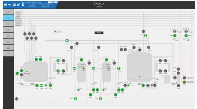
Overview of the chocolate production line.
