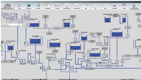
Figure 1: With the zenon Worldview, the LFWV technicians always have access to the entire equipment – even when they are not on site.
